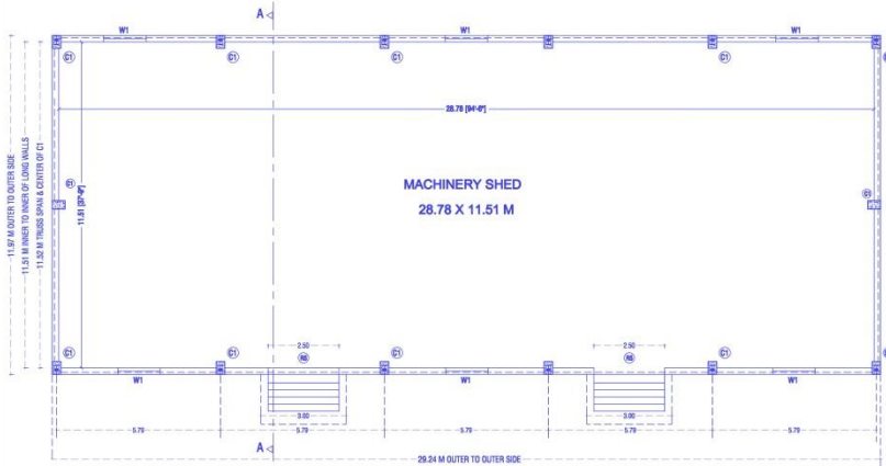
MACHINERY SHED PLAN
