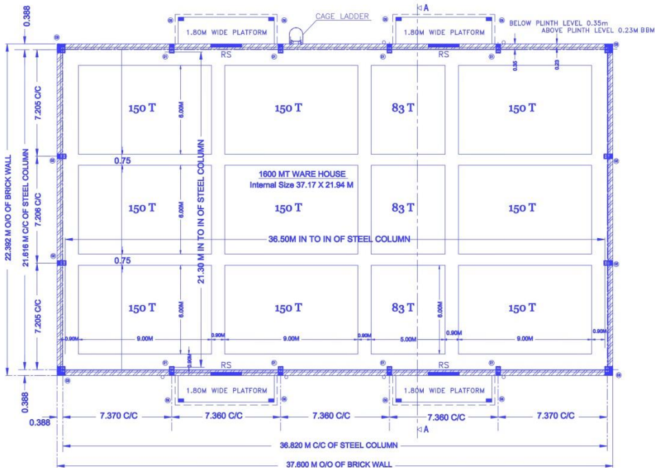
PLAN FOR 1600 MT WARE HOUSE UNIT
